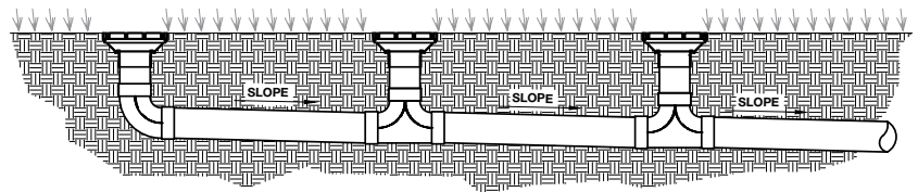
LOW PROFILE ADAPTER - LANDSCAPE APPLICATION
