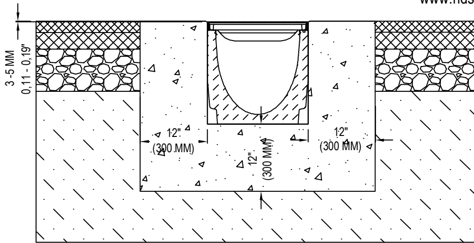
SECTION
