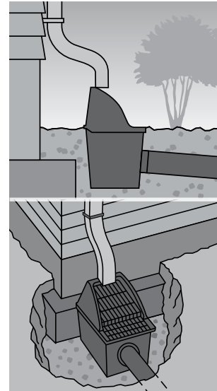
Figure 2 Downspout with return elbows
