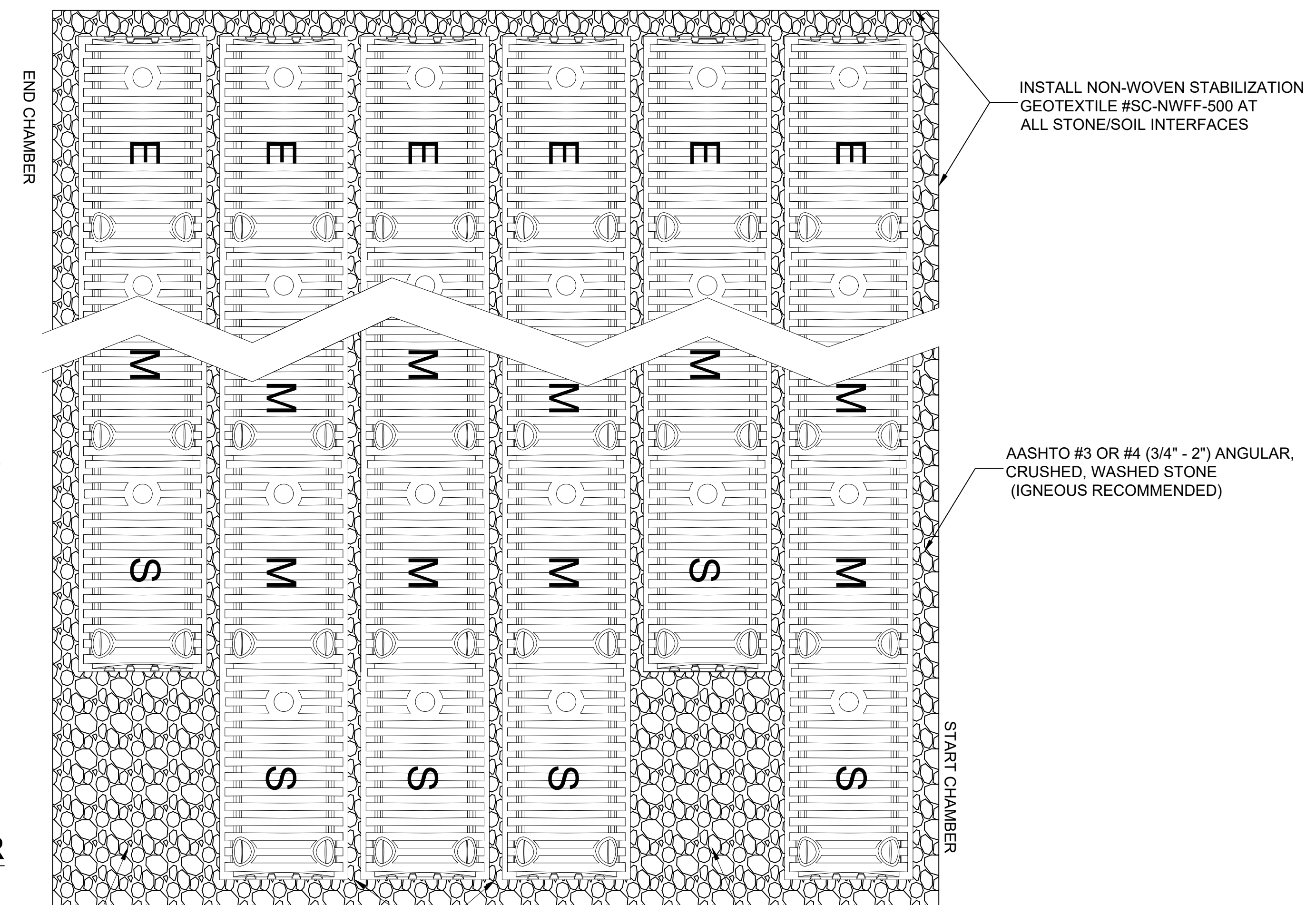
PLAN VIEW TOP LAYER
