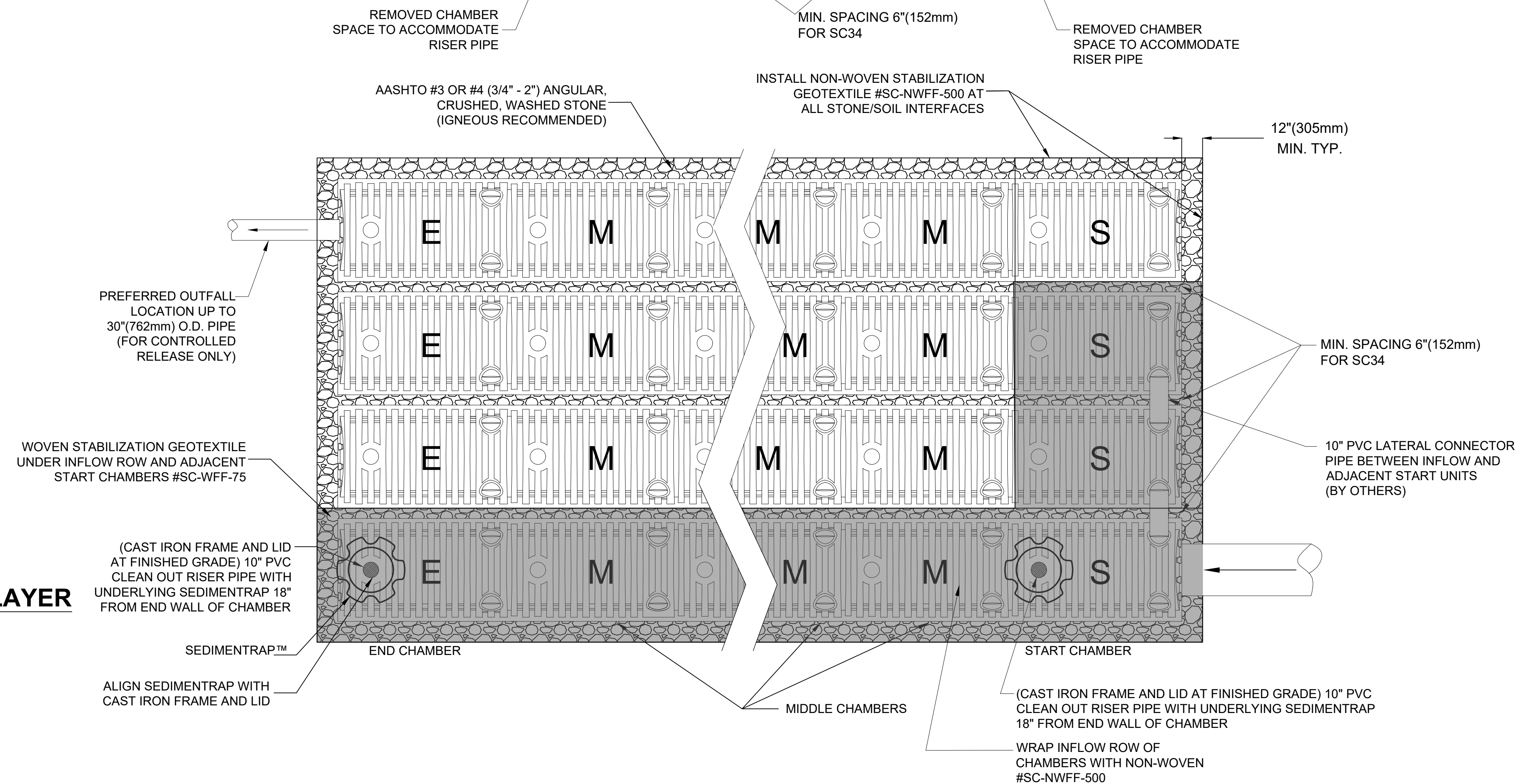
PLAN VIEW TOP LAYER
