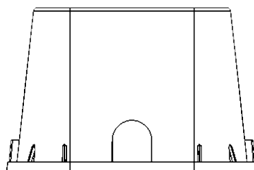
View A-A Pipe Slot 2 7/8" x 3 5/8"
