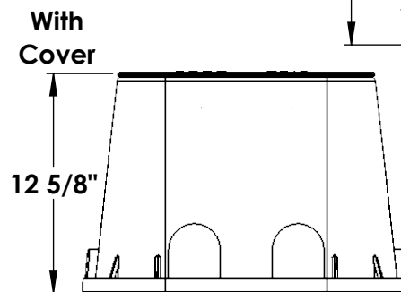
Dual Pipe Slot 2 7/8" x 3 5/8"
