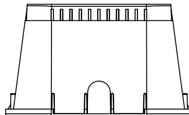
View A-A Pipe Slot 2 1/2" x 3 1/2"
