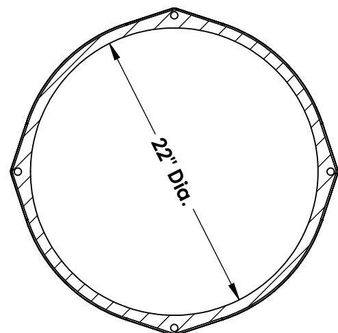
View B-B
